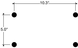
Mounting Pattern
